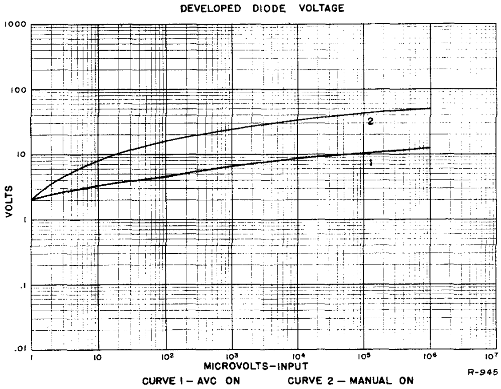
Figure 20--AVC Curves
