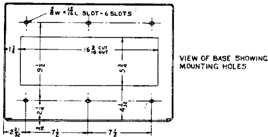
OUTLINE DIMENSIONS OF 9-AX CABINET RACK
