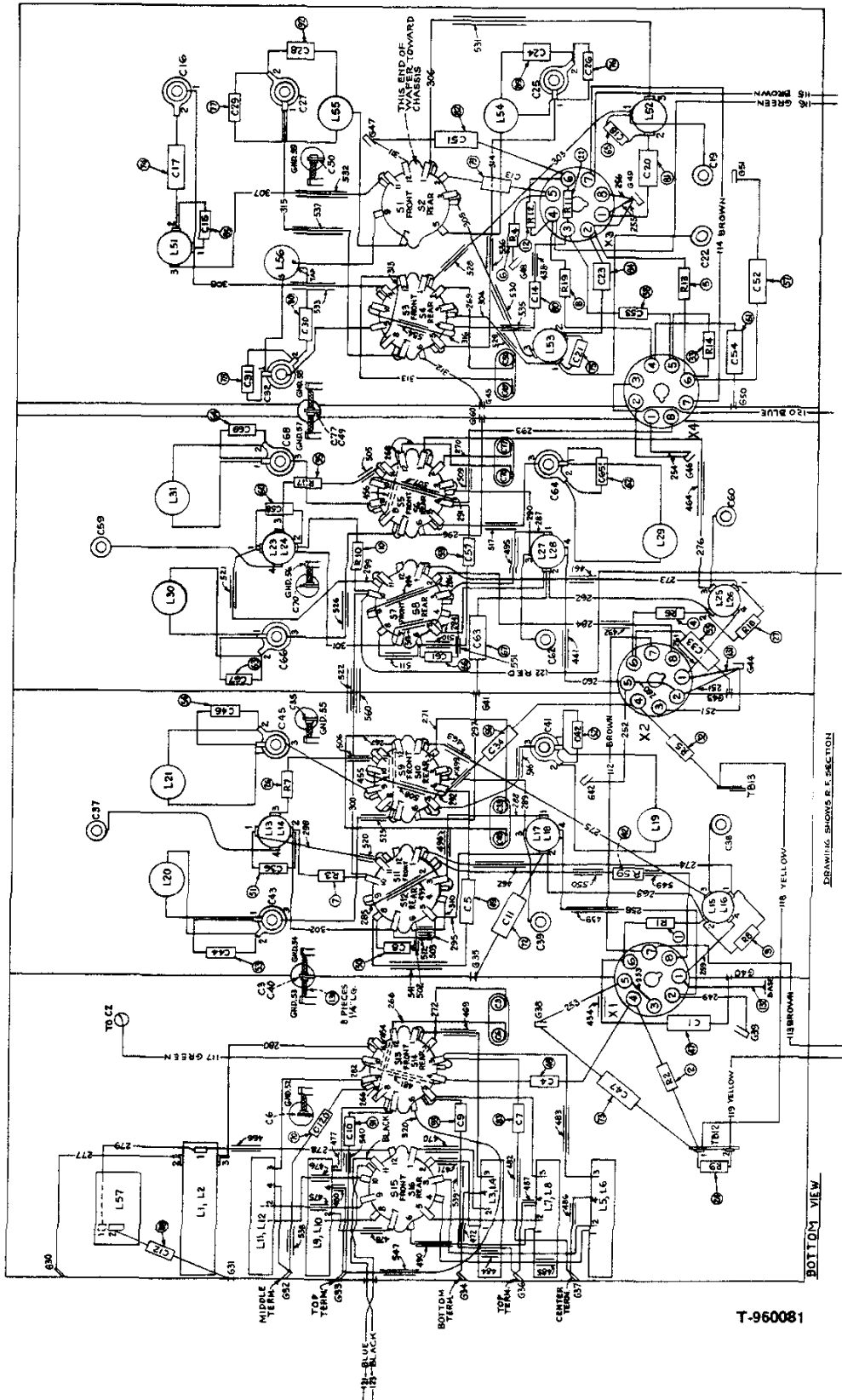
Figure 22—Connection Diagram (R-F Unit, Bottom View)
