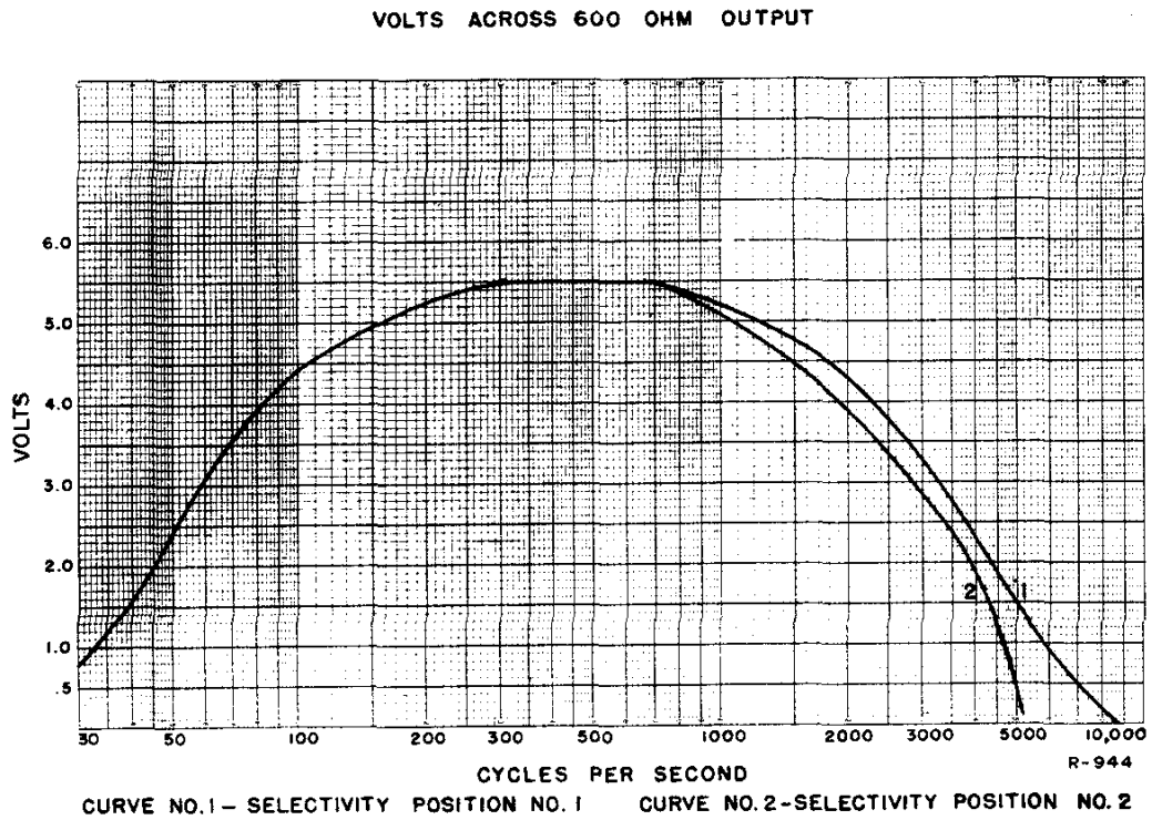
Figure 19—Fidelity Curves
