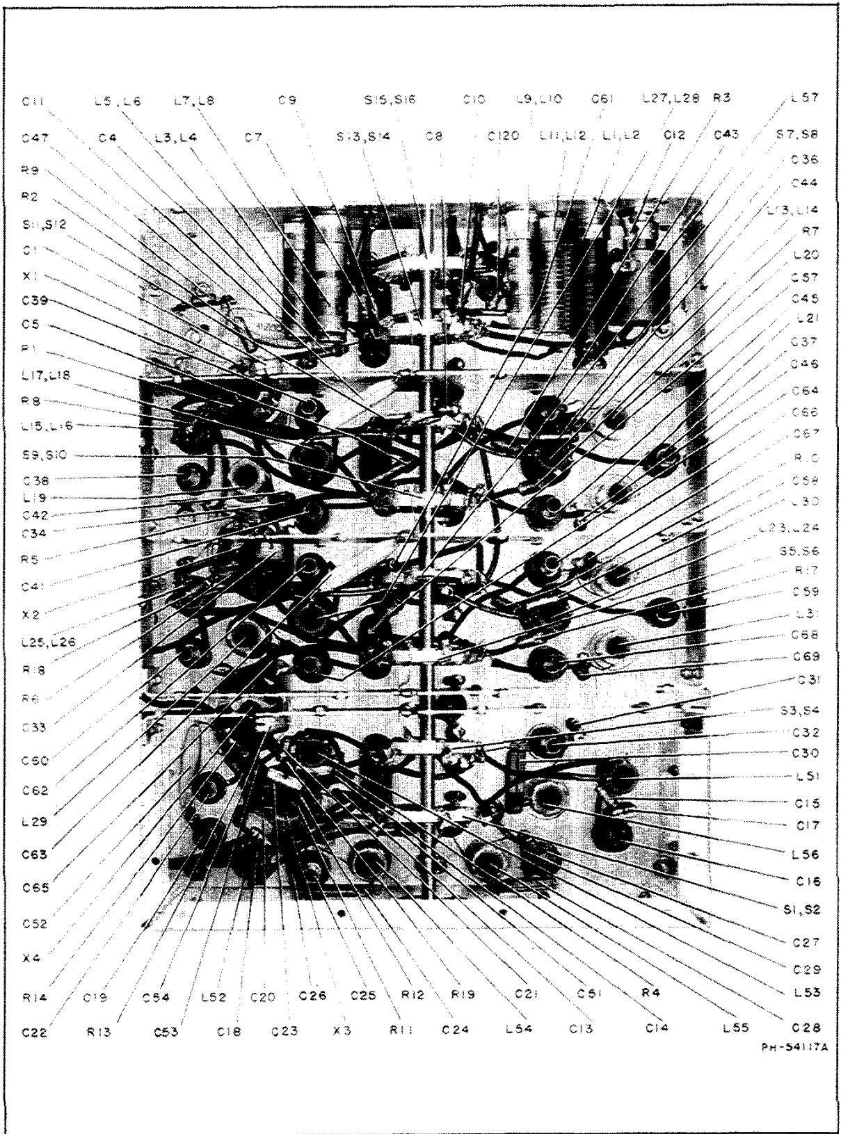
Figure 16-- R-F Unit
